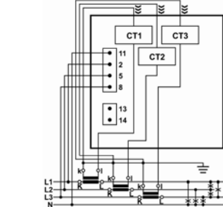
4u – four-wire, non-uniform load
