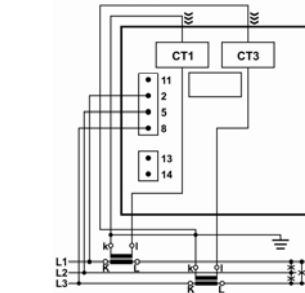
3u – three-wire, uniform load
