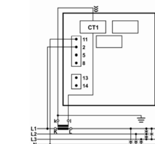
4b – four-wire, uniform load
