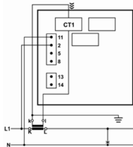
1b – single-wire, uniform load
