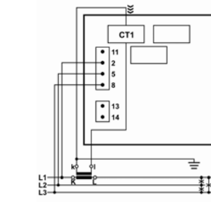
3b – three-wire, non-uniform load
